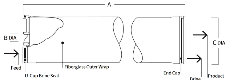
FilmTec™ supplies coupler part number 313198 with each element. Each coupler includes two 3-912 EPR O-rings (part number 151705).
